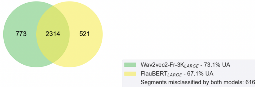
Fig. 5. Correct classifications for the 2 models on our dataset (4224 samples), i.e. Wav2vec2-FR-3K LARGE (Convolutional layers frozen) correctly classified (773 + 2314)/4224 \equiv 73, 1\% UA.
