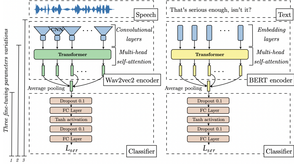
Fig. 2. Three variations of fine-tuning of the learning parameters: (1) No encoder fine-tuning, (2) Convolutional layers (wav2vec) / Embedding layers (BERT) frozen, (3) Full fine-tuning.
