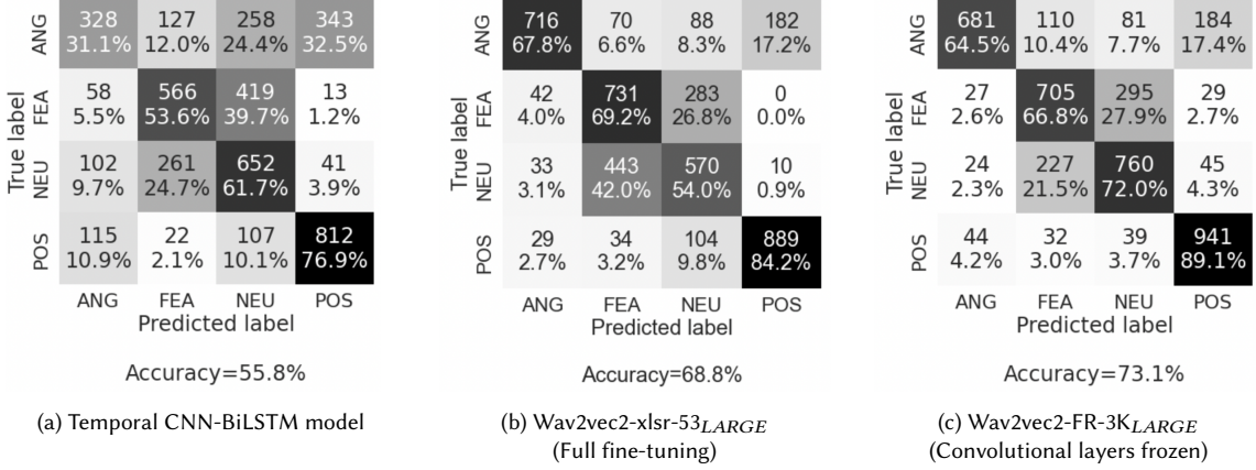
Fig. 4. Confusion matrices of three speech emotion recognition models with CEMO
