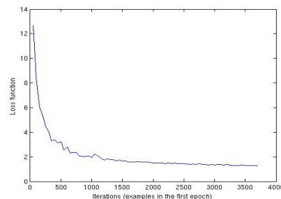
Figure 1: Perceptron loss on training data
