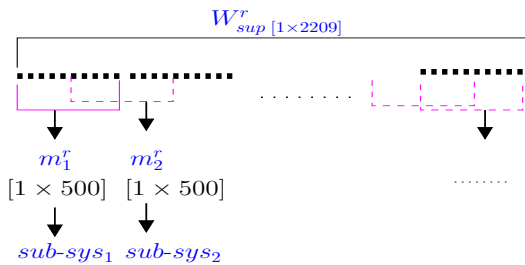
Figure 1: m -vector extraction of r^{th} speaker from his/her MLLR super-vector using an overlapped window of 500 elements.
