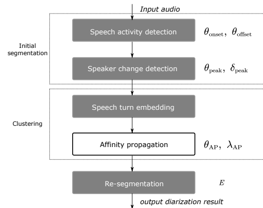
Figure 1: Proposed diarization pipeline and hyper-parameters. Modules with gray background are based on neural approaches.
