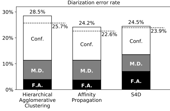
Figure 3: Performance on ETAPE TV test set. Black bars, gray bars and white bars indicate false alarm, miss detection and confusion respectively. Dashed lines indicate performance when tuned on test set.
